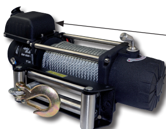
Standardmodell
